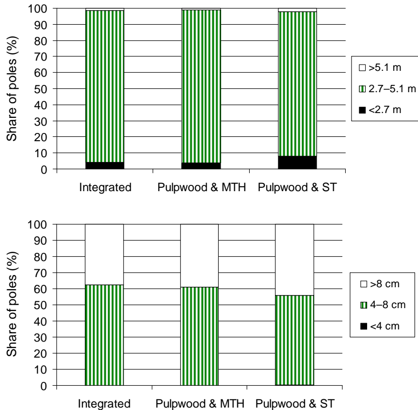
Figure 5. The length and top diameter distributions of bucked pulpwood poles by tested cutting method at Loppi.
